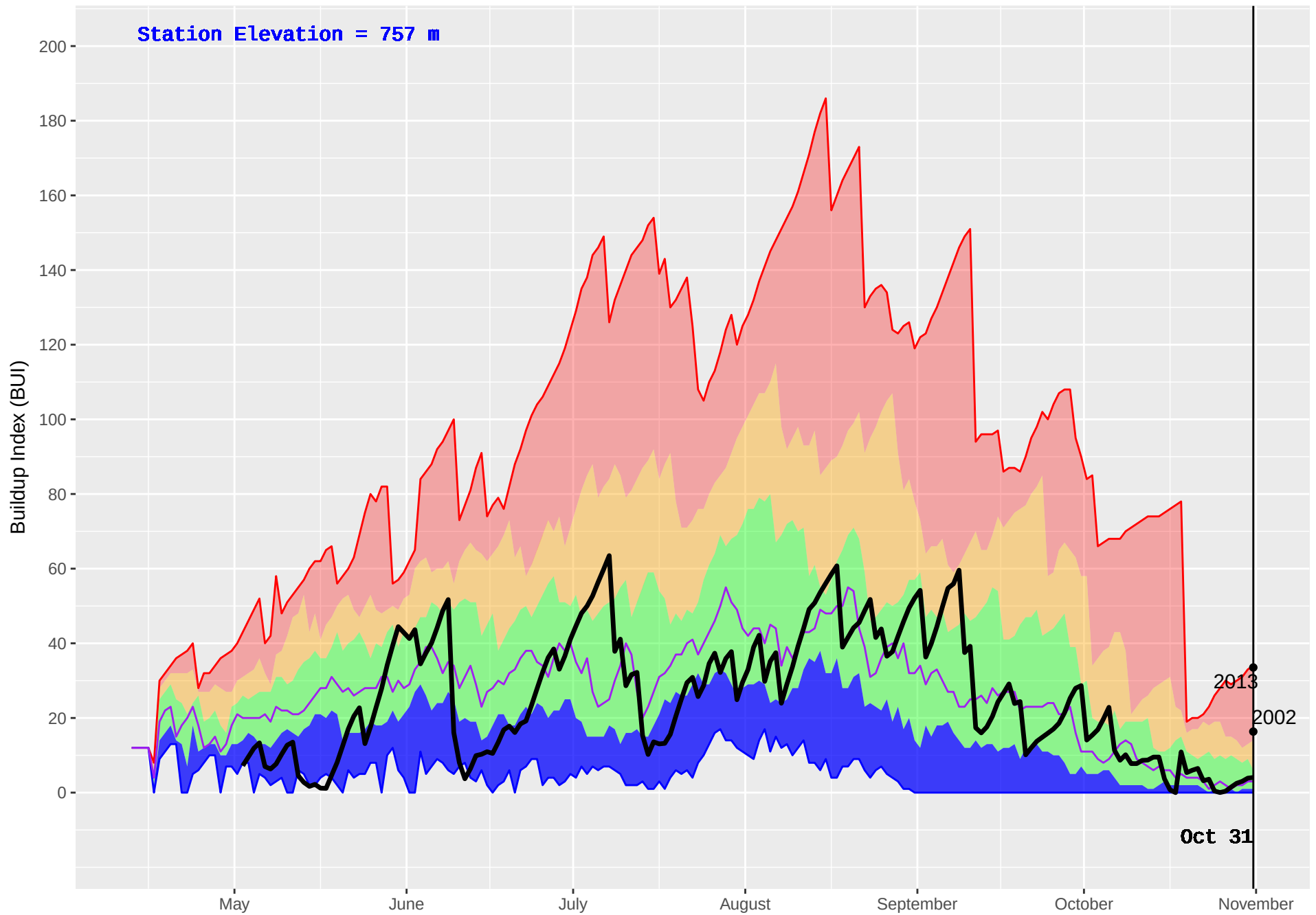
LEMORAY (140) : Historical (1988–2016) and Current (2017) Noon Buildup Index (BUI)
